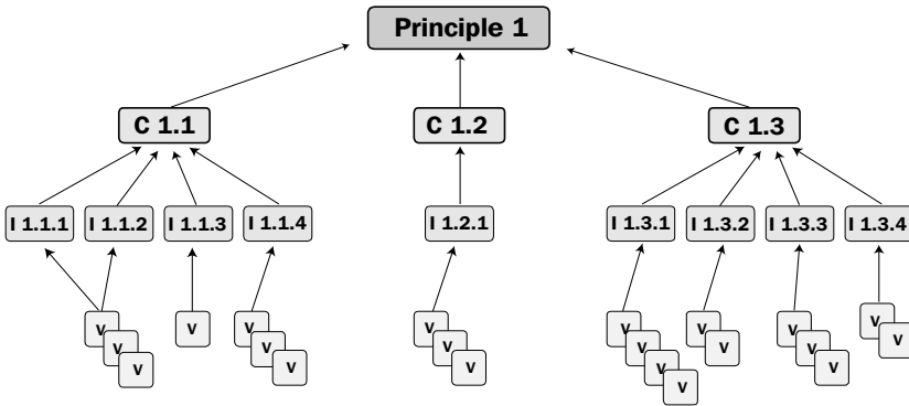
Figure 1. Hierarchical structure.
